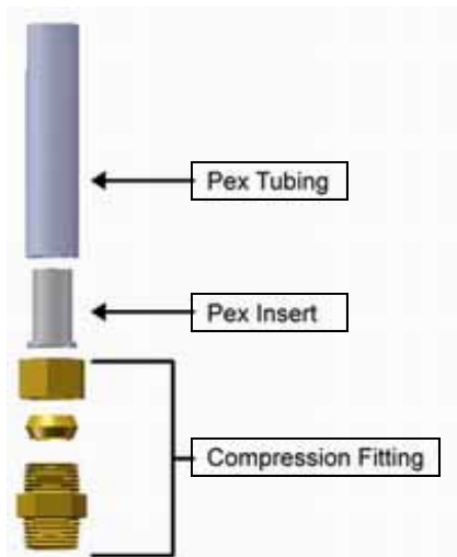
Compression Fitting Components
