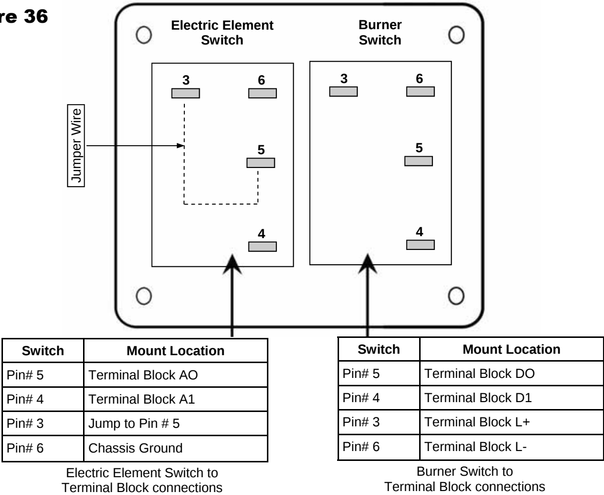
Interior Switch Panel, Rear View
