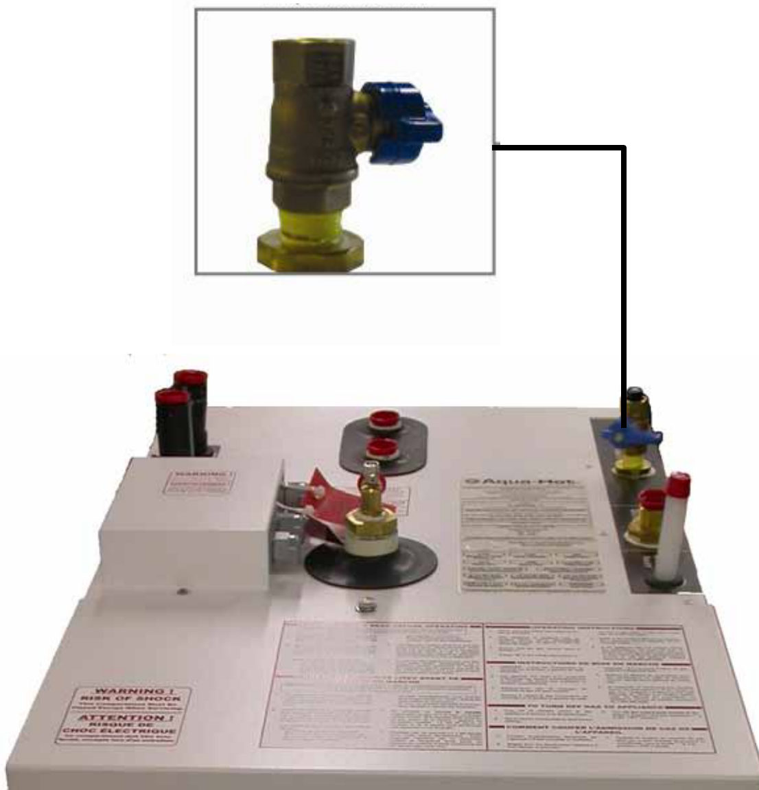
Manual Shut-Off Valve for Propane Supply Installed in Propane Inlet Port
