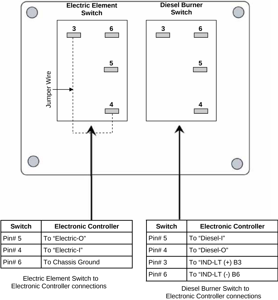
Figure 36 Aqua-Hot 400D Switch Panel, Rear View
