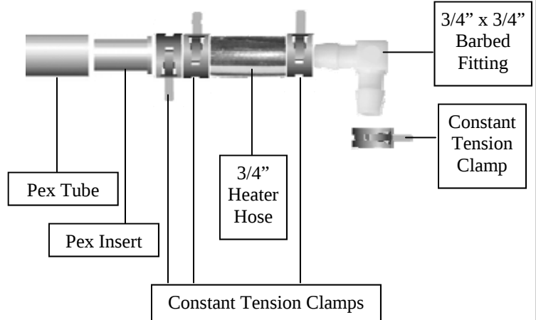
90° Connection Components
