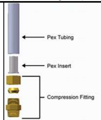
Compression Fittings Components
