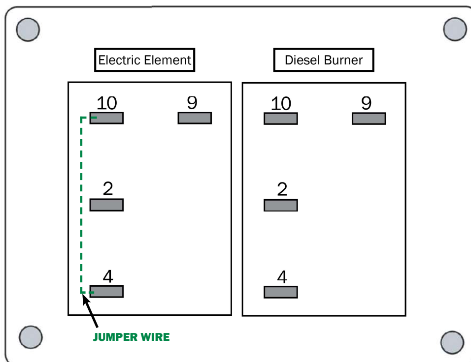
Switches Rear View
