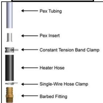
Barbed Fittings Components
