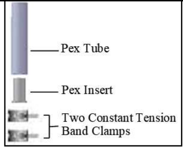
Barbed Fittings Components Installed
