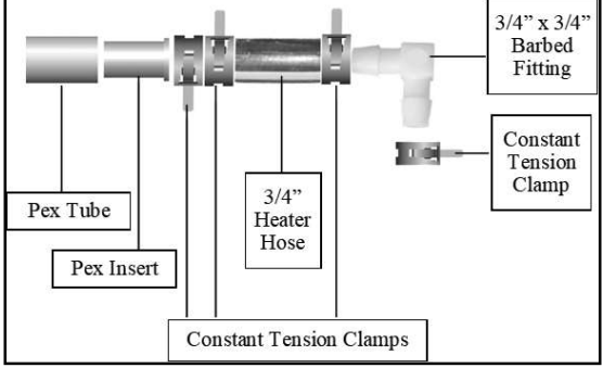
Compression Fittings Components Installed
