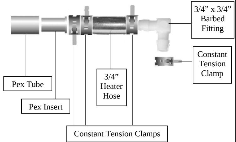
90° Connection Components
