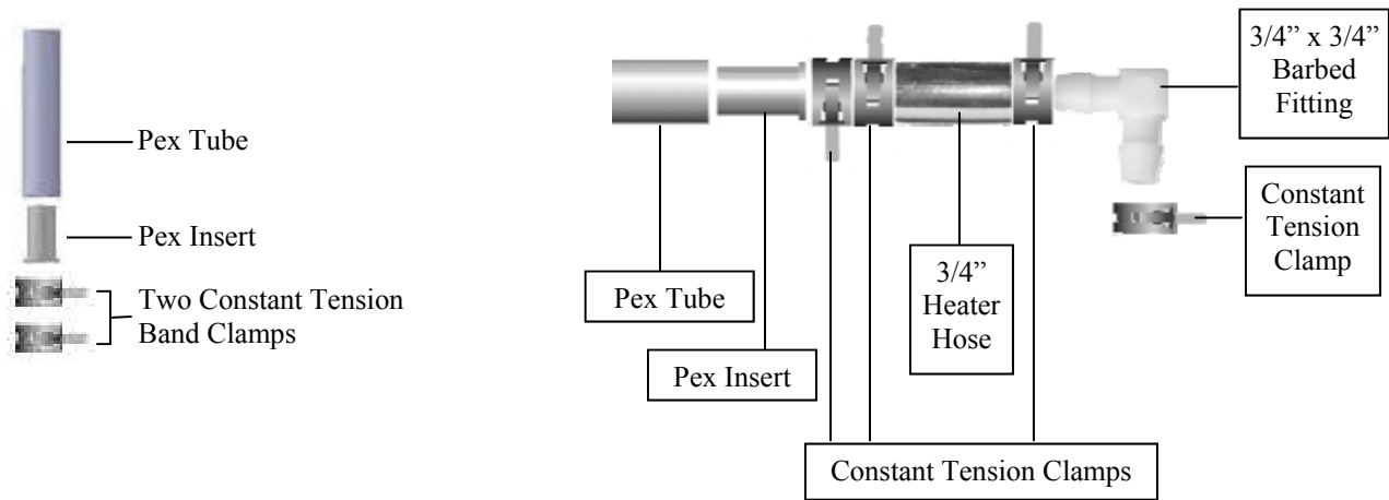
Straight Connection Components
