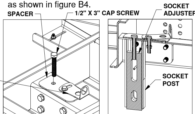
Figure B3: View of center of base
