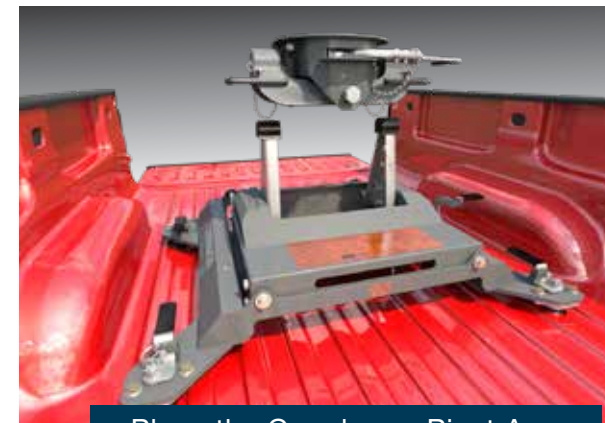
Place the Coupler on Pivot Arms
