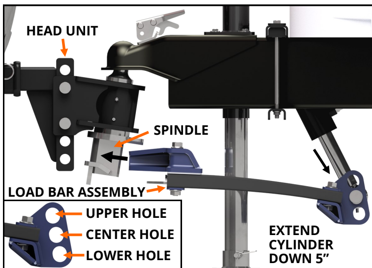
FIGURE G2: View of the driver side of the hitch.
