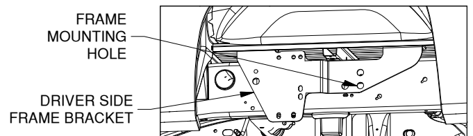
Figure A3: View looking into driver side wheel well.
