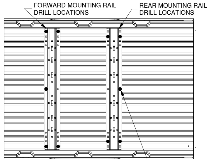
Figure B2: Detail view over bed, showing drill locations for the forward and rear bed rails.
