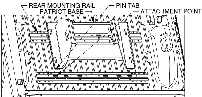
Figure E3: View into truck bed looking back at tailgate.
