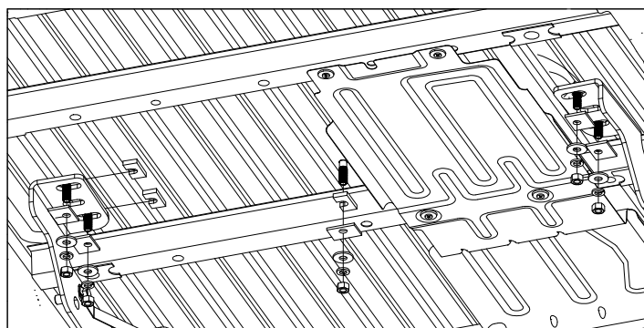
Figure D2: View under bed looking up toward cab. (Frame not shown)
