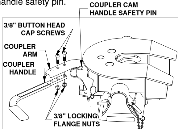
Figure D1: View looking down at side of coupler head.
