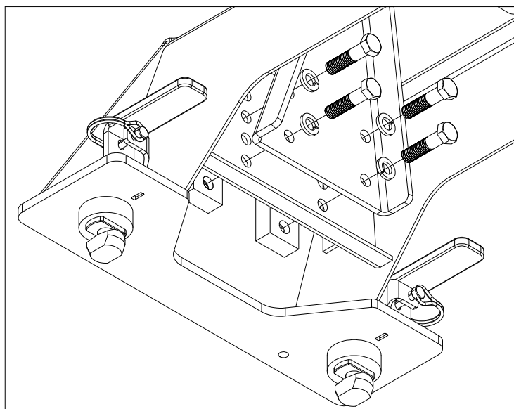
Figure A2: Passenger pivot arm mounting location.
