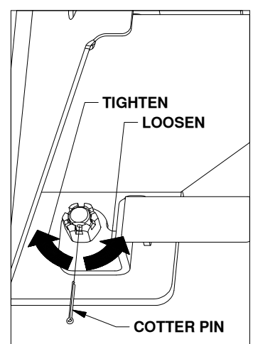
Figure C4: View of base leg.
