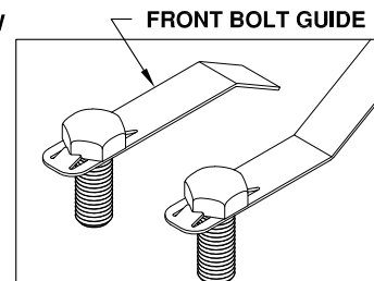
Figure C2: Bolt Guides
