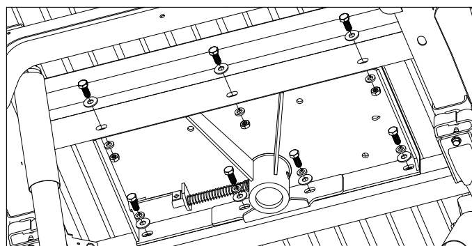
Figure B6: View under bed of hardware assembly.
