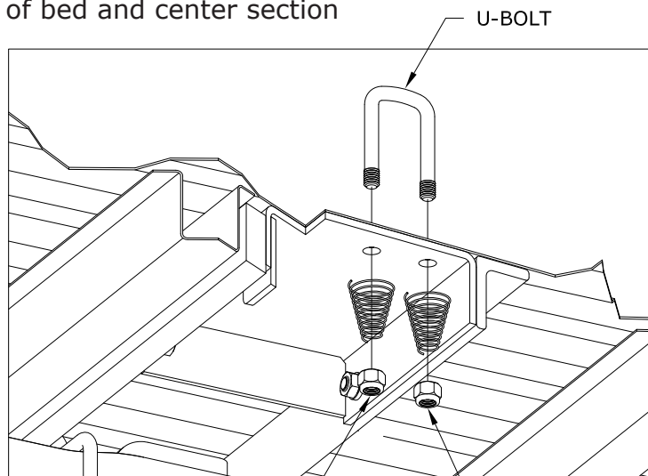
FIGURE 6.3: Cut away view from under the bed
