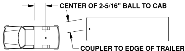
Figure A2: Truck and trailer diagram
