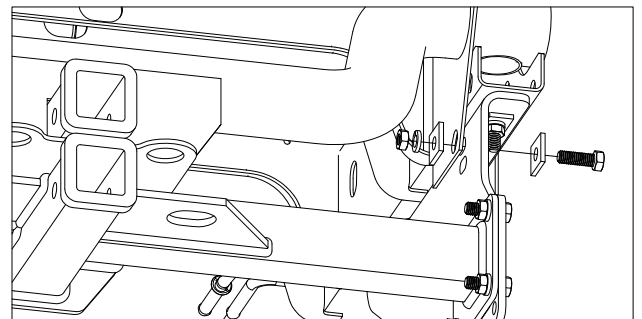
FIGURE 4.1: View looking at passenger side of frame looking towards the cab. (bumper and bed not shown)
