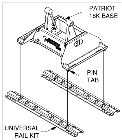
Figure B1: Rail Attachment
