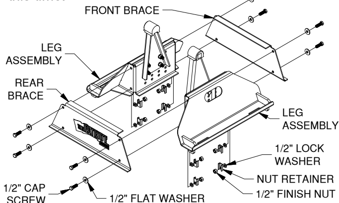
Figure A4: Base assembly.
