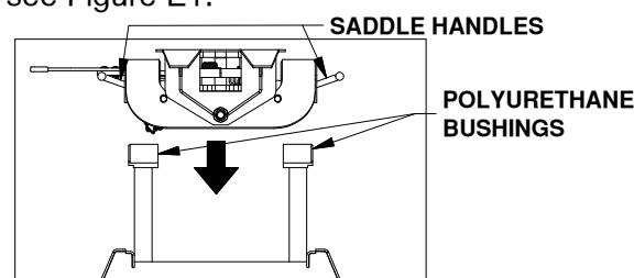
Figure E1: View of coupler and base. (Saddle Handles up)
