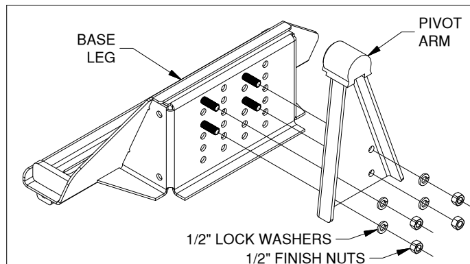
Figure A3: Base Leg and pivot arms.
