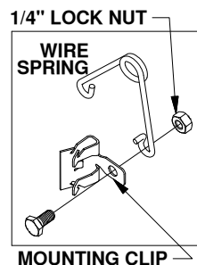
Figure C1: Leveling kit parts.
