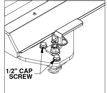
Figure B4: View of base foot
