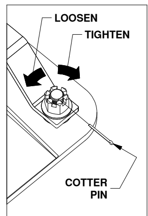
Figure C4: View of base leg.
