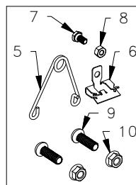
COUPLER BOLT BAG (RVC3006)
