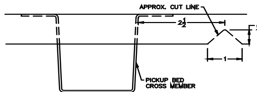
BED FLOOR FLANGE IN PASSENGER'S SIDE WHEEL WELL
