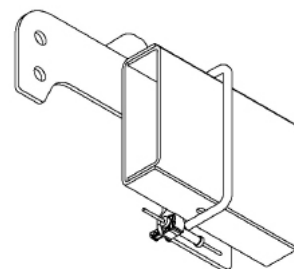
Side plate installed and clip in place.
