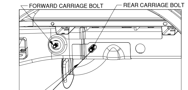
Figure C2: View of driver side wheel well.
