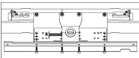
Figure E3: Looking up at center section. (Frame not shown.)
