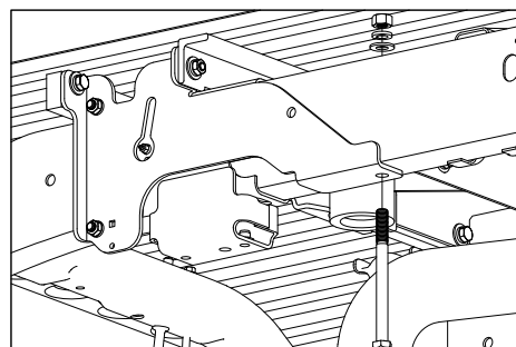
FIGURE 4.5: Driver side of frame.
