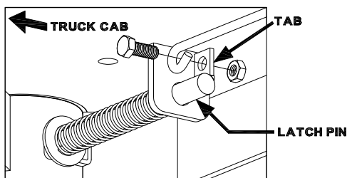
FIGURE 6.2: Handle installation
