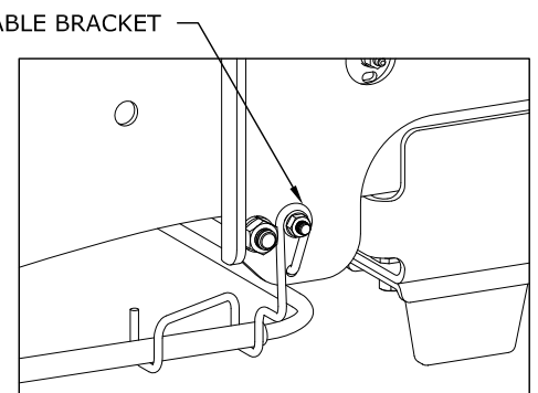
FIGURE 4.6: Cable Bracket
