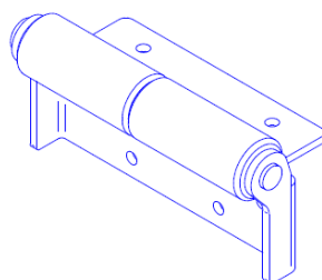
854303 AFTERMARKET ROLLER USED TO ASSIST 3/4" WEAR BAR
