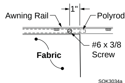
Figure 17. Fabric Attach.
