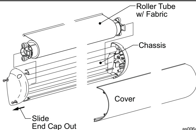
Figure 5. Unpacking the Unit.
