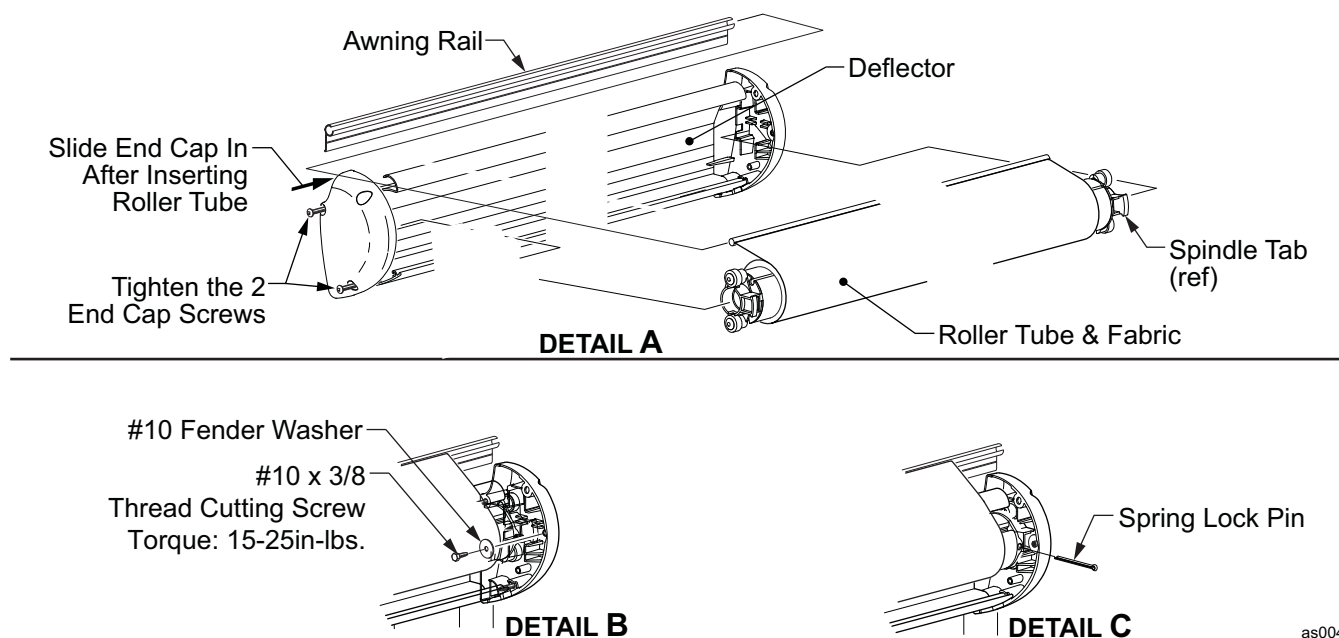
Figure 9. Installing the Roller tube Assembly.
