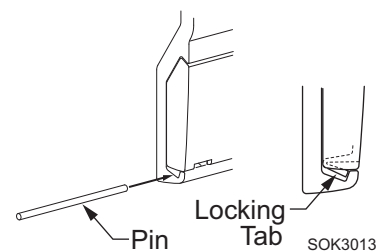
Figure 14. Removing the Cover.
