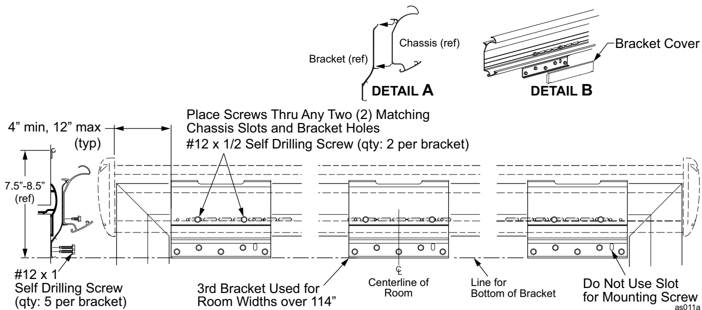
Figure 7. Mounting the Deflector w/ Brackets.
