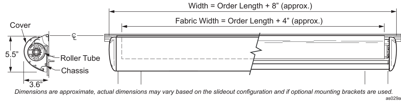
Figure 1. General Dimensions.
