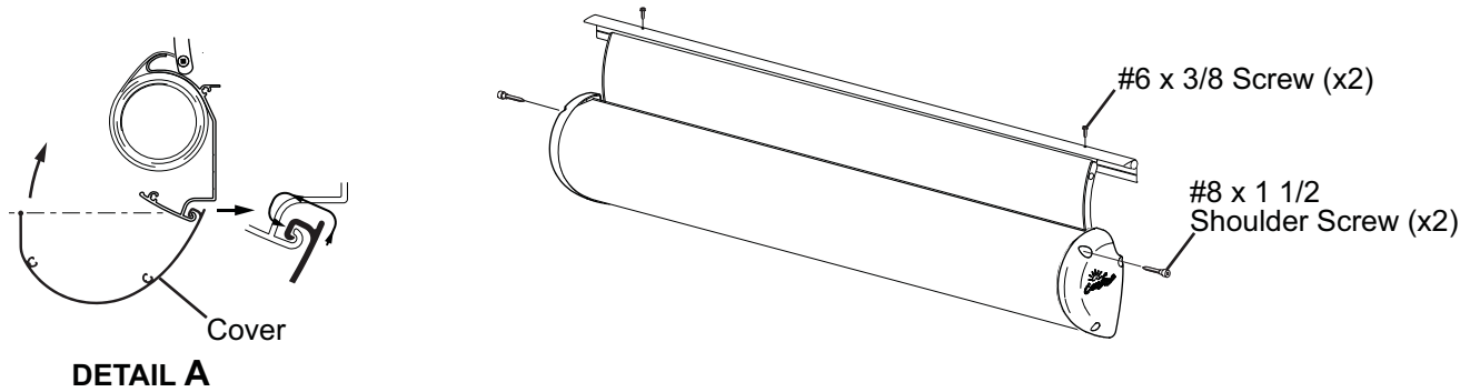
Figure 11. Installing the Cover.
