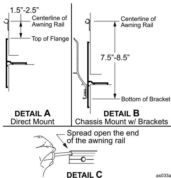
Figure 4. Mounting the Awning Rail.
