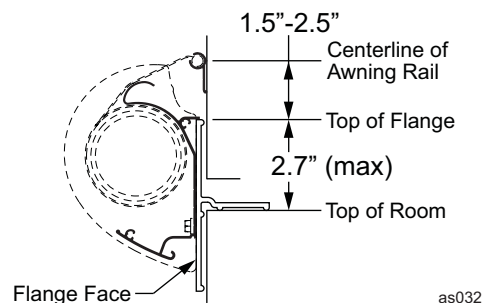
Figure 2. Direct Mount of Deflector.
