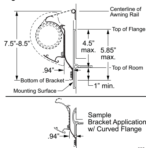
Figure 3. Deflector Mount w/ Bracket.
