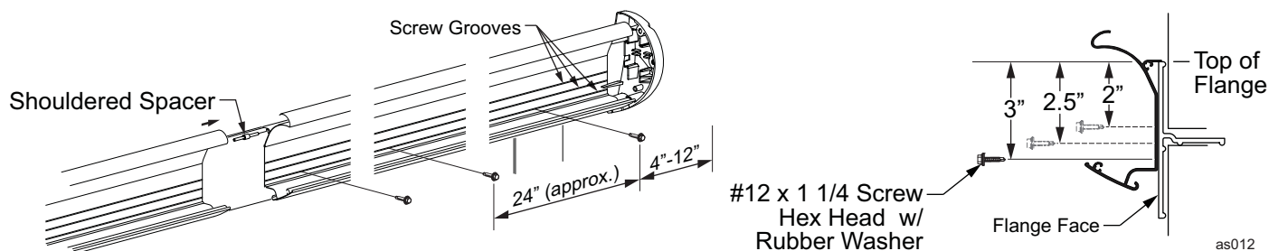
Figure 12. Installing the Deflector.
