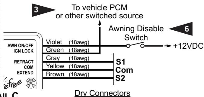
DETAIL C Multiplex Control System
