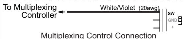
DETAIL B Awning Lights Switch Options
