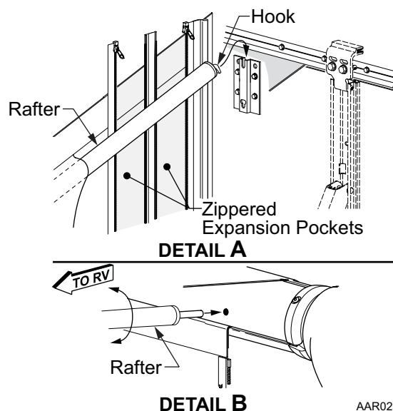
Figure 7. Attaching the Rafter.
