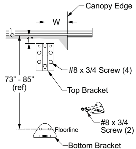
Figure 3. Installing the Snapless Brackets.
