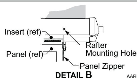
Figure 4. Installing the Front Panels - Manual Awnings.
