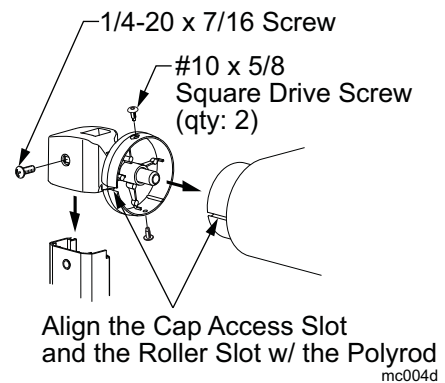
Figure 4. Attaching the Idler End Plug.
