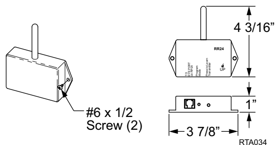
Figure 10. RR24 RF Receiver.
