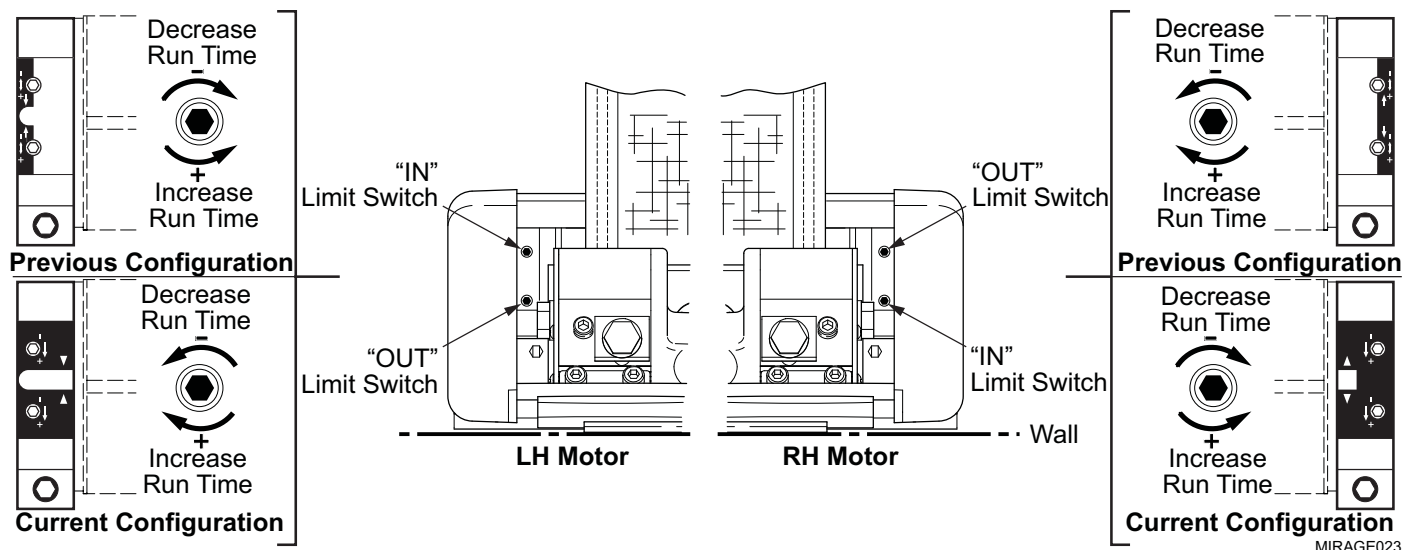
Figure 15. Motor Limit Switches.
