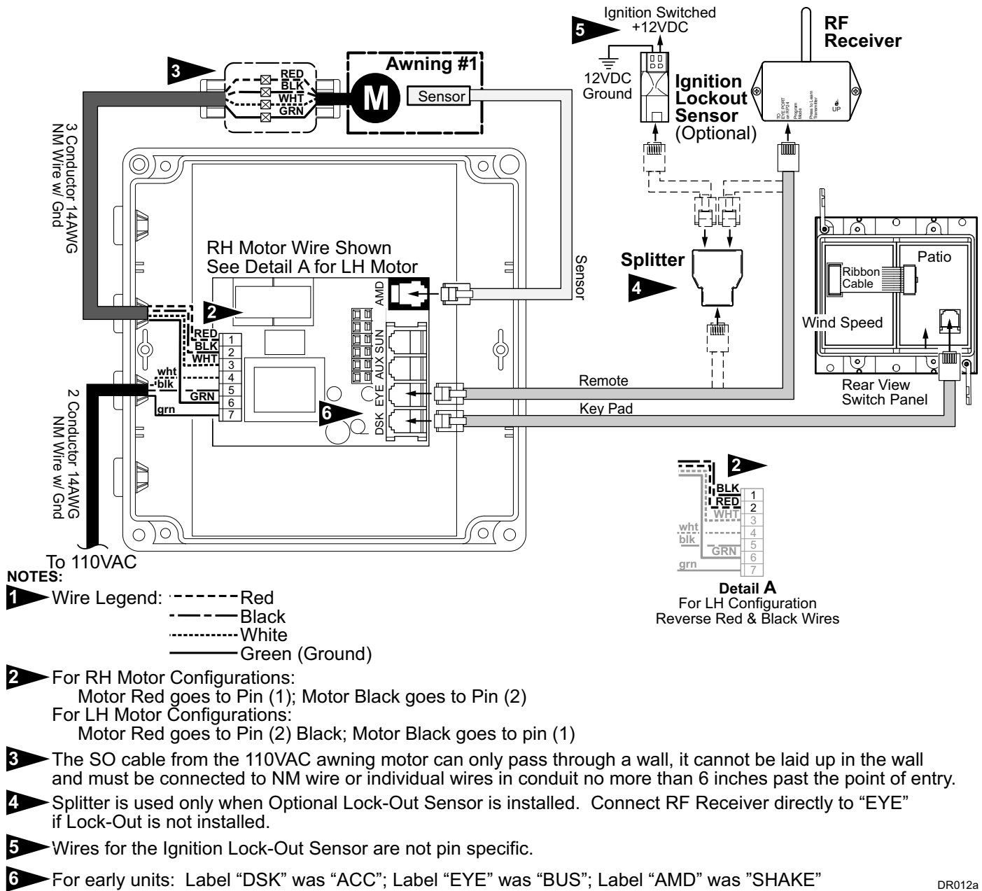
Figure 12. Wiring Diagram – Direct Response System.
