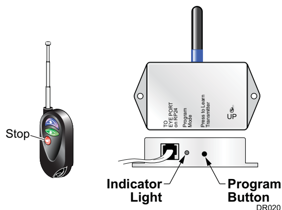
Figure 11. RF Receiver.
