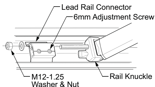
Detail A (Lead Rail)
