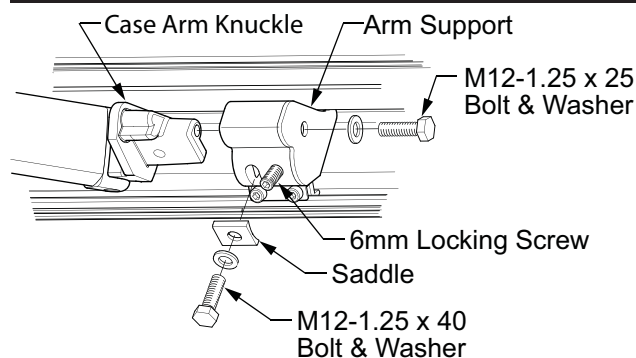
Detail B (Case)
