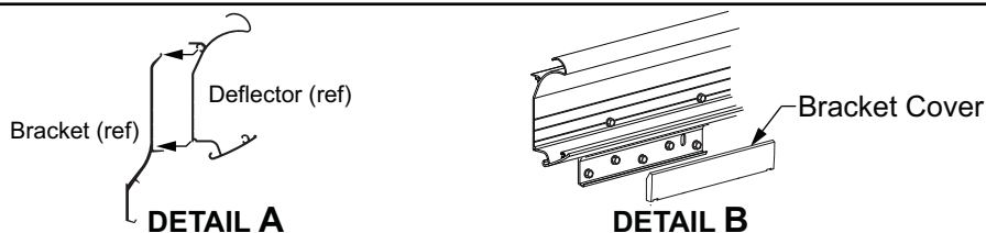
Figure 7. Mounting the Deflector w/ Brackets.
