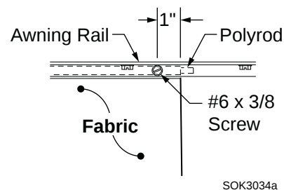
Figure 17. Fabric Attach.
