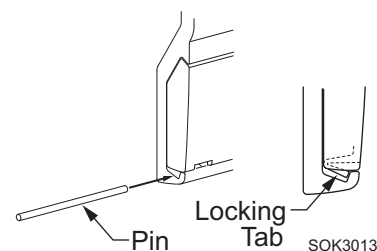
Figure 8. Removing the Cover.
