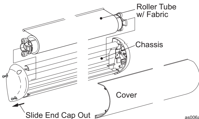
Figure 5. Unpacking the Unit.
