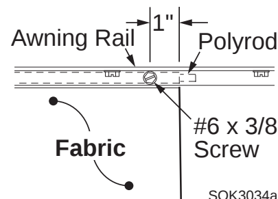
Figure 10. Securing the Fabric.
