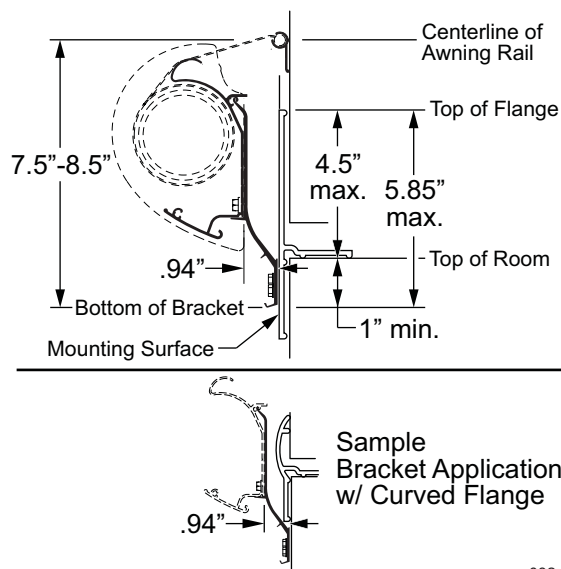
Figure 3. Deflector Mount w/ Bracket.
