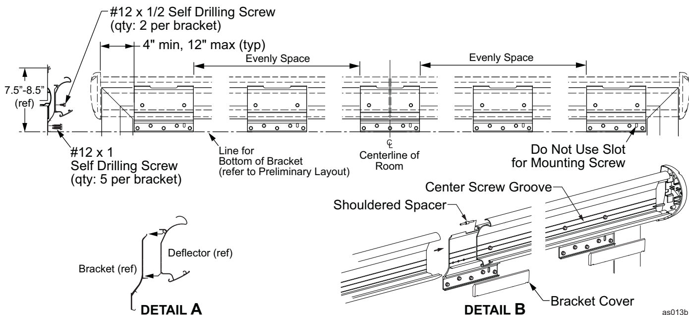
Figure 13. Mounting the Deflector w/ Brackets.
