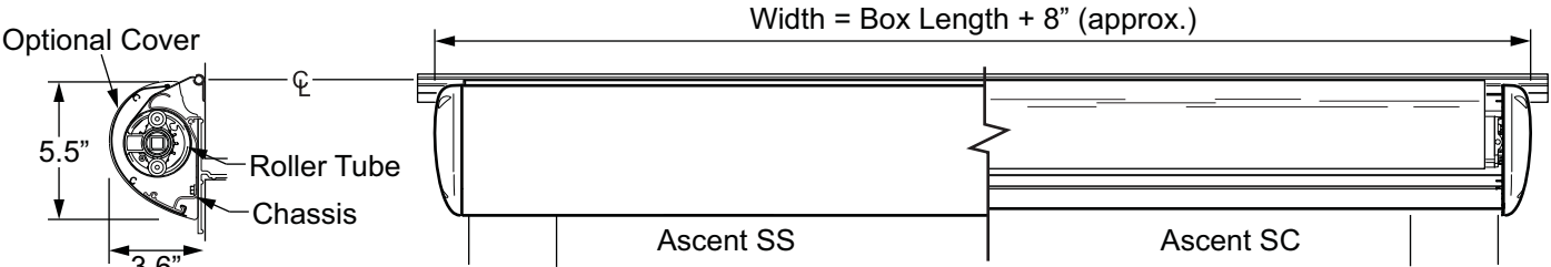
Dimensions are approximate, actual dimensions may vary based on the slideout configuration and if optional mounting brackets are used. as029a
