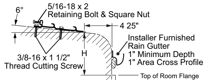
Directly Mounting to the Coach Roof
