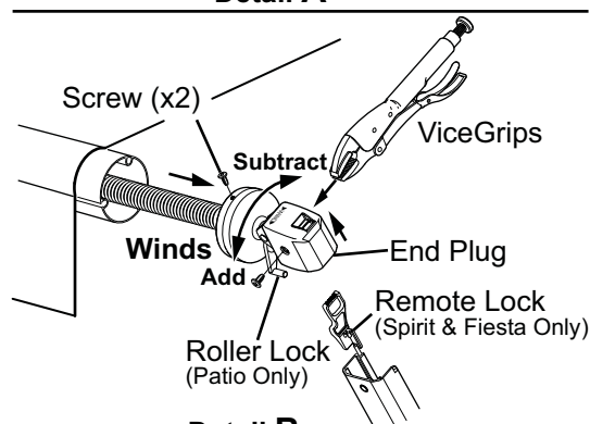
Detail B
