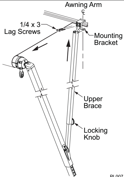
Figure 5. Upper Bracket.
