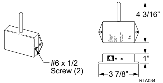
Figure 1. RF Receiver.
