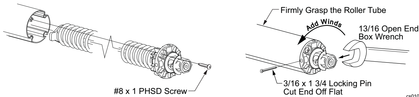
Figure 2. Replacing the Spring Assembly.
