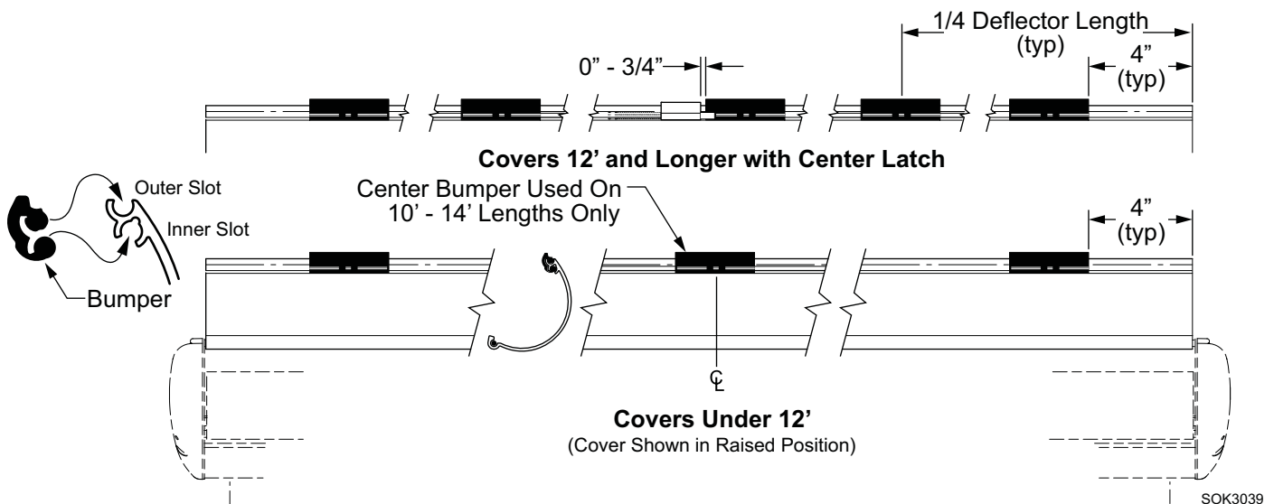
Figure 10. Cover Bumpers.
