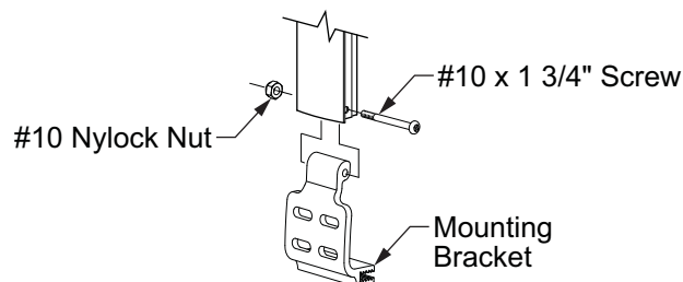
Lower Mounting Bracket
