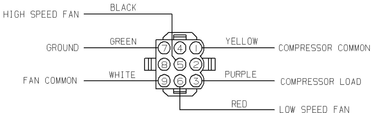
Figure 7. High Voltage 9-Pin Connector
