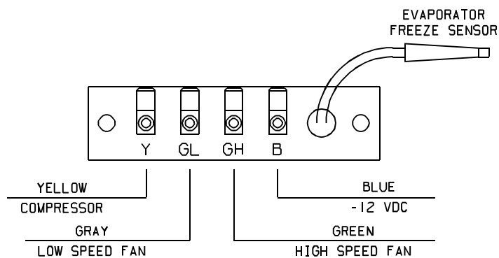
Figure 6. Low Voltage Terminal Strip
