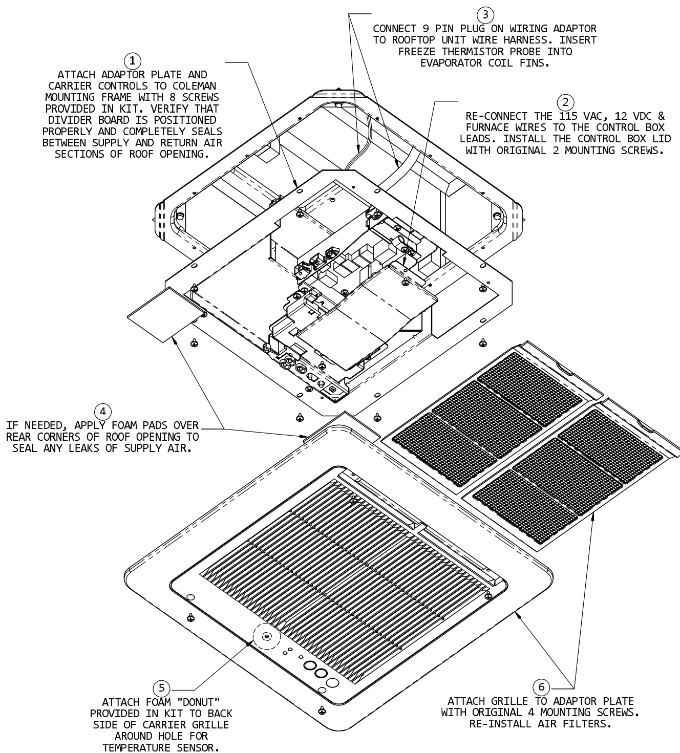
FIGURE 5 FINISHING INSTALLATION
