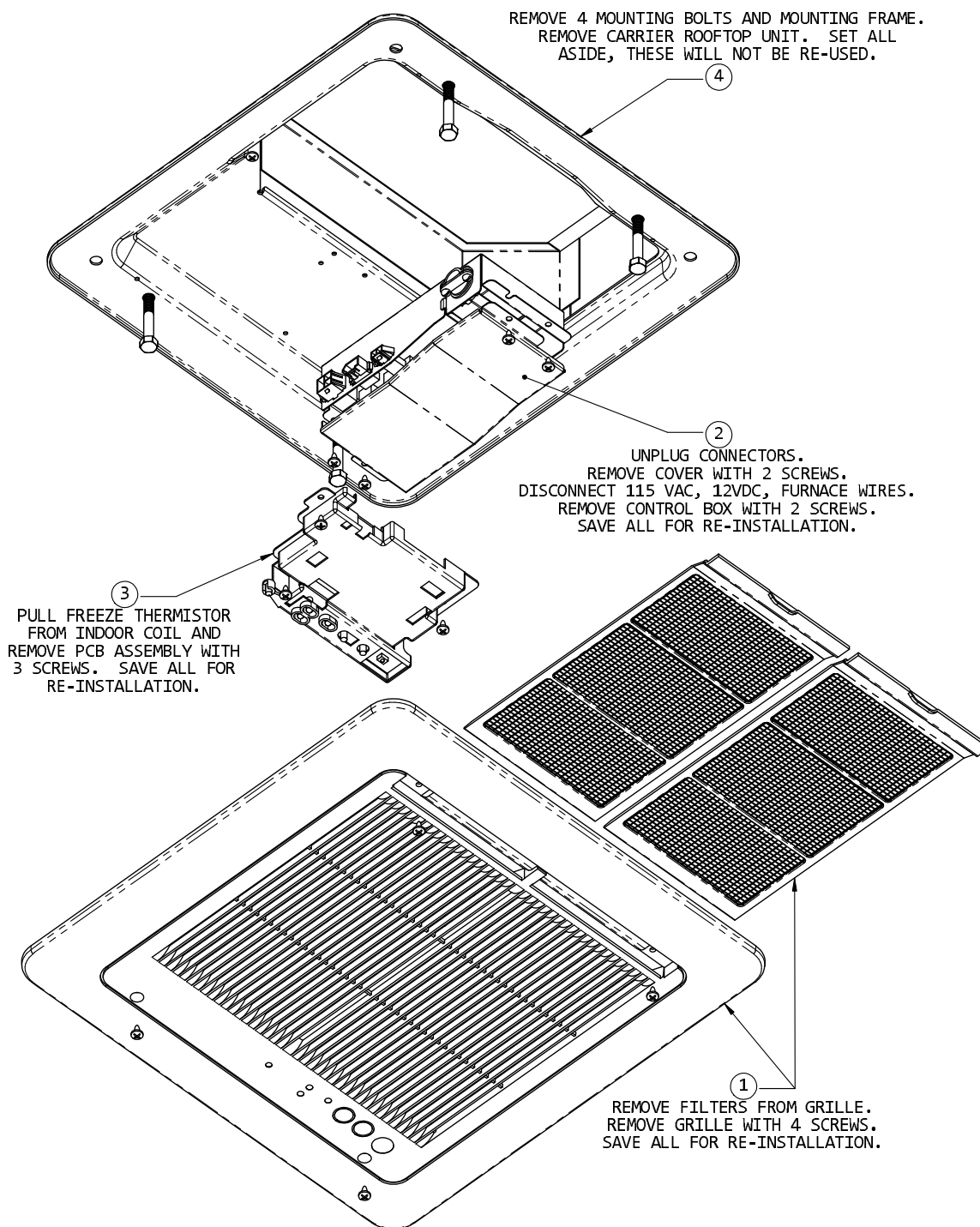
FIGURE 1 CARRIER UNIT REMOVAL PROCEDURE
