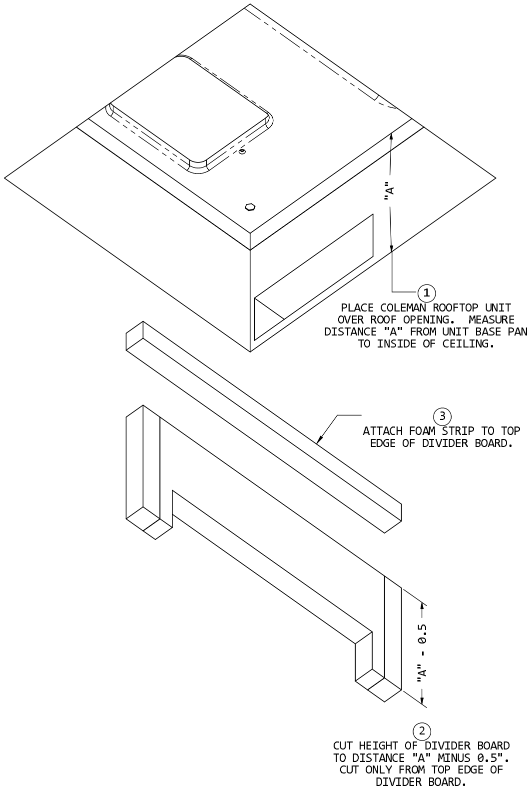
FIGURE 2 FITTING COLEMAN DIVIDER BOARD
