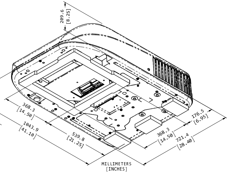
47103*79X5 & 47103*79X7 16" Gasket version fits 14" or 16" openings.
