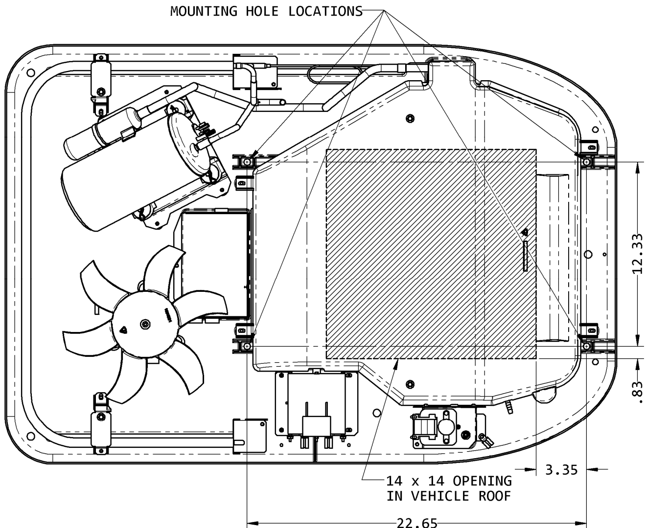
TOP VIEW OF MACH 8 UNIT WITH SHROUD REMOVED
