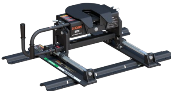
16616 - E16 head with R16 roller and base rails
