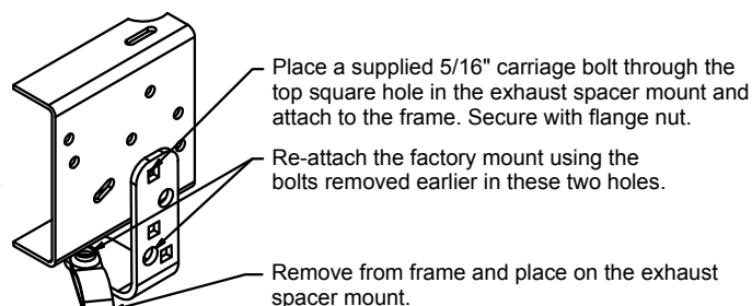
FIGURE E (EXHAUST MOUNTS WITH TWO BOLTS)
